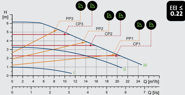
MAGNA1 50-60 F (N)
