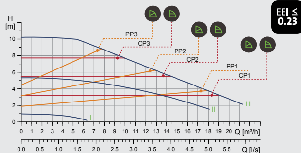
MAGNA1 40-100 F (N)
