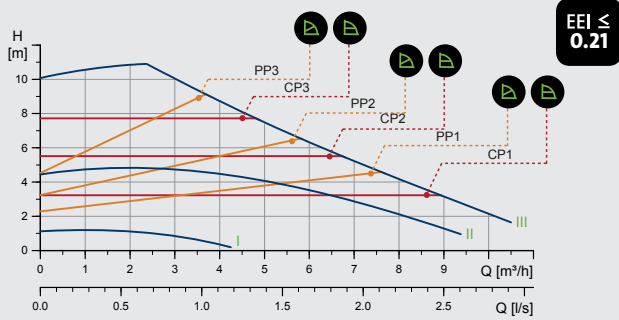
MAGNA1 32-100 F (N)
