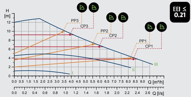
MAGNA1 32-120 (N)
