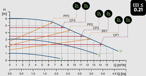
MAGNA1 40-60 F (N)
