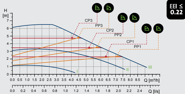
MAGNA1 32-60 (F) (N)
