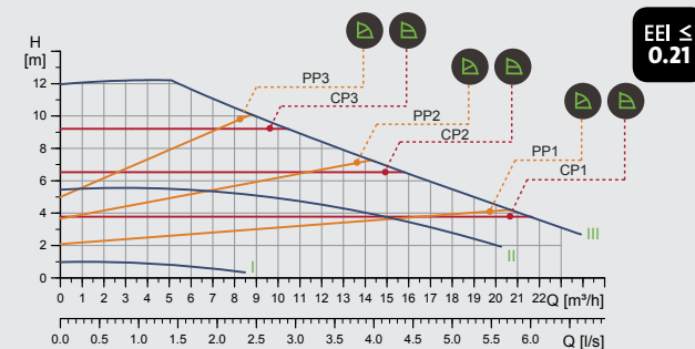
MAGNA1 40-120 F (N)
