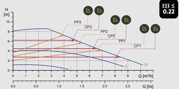
MAGNA1 32-80 (F) (N)
