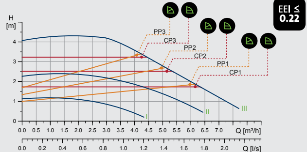
MAGNA1 32-40 (F) (N)
