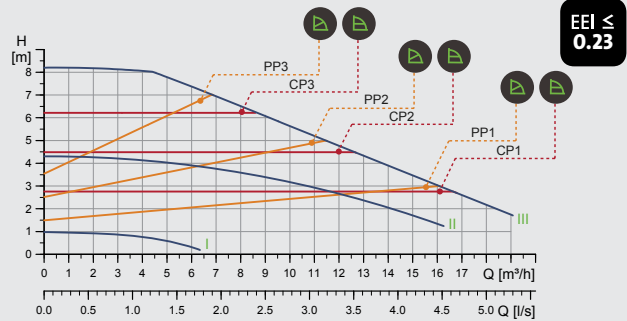
MAGNA1 40-80 F (N)
