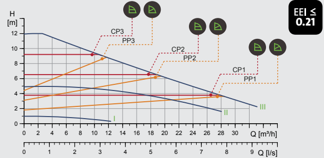
MAGNA1 50-120 F (N)
