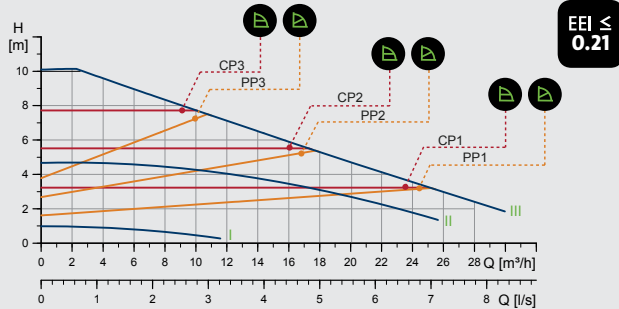
MAGNA1 50-100 F (N)
