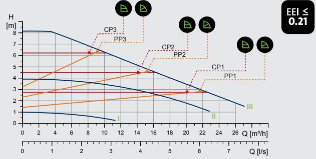
MAGNA1 50-80 F (N)
