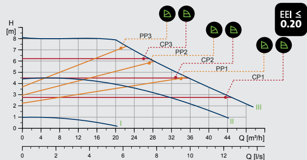
MAGNA1 80-80 F
